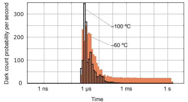
FIG. 2. Dark count probability versus time elapsed since a count, at -60 and -100^\circ\text{C} . The first 0.5 \mu\text{s} is deadtime; the peak is caused by afterpulses; the count probability settles to the dark count rate at long time values.
