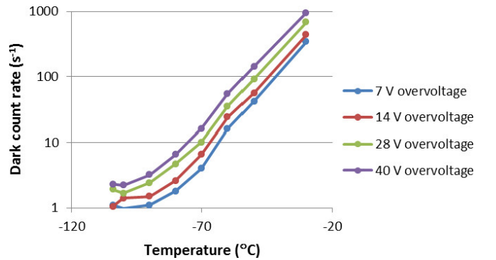
FIG. 1. Dark count rate of Si-APD vs. temperature, at four different voltages above breakdown voltage.
